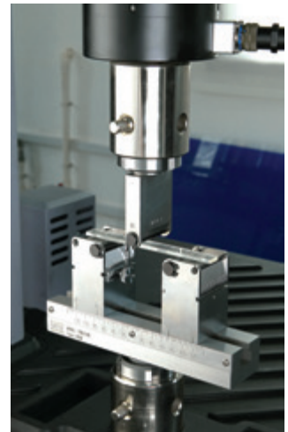
Bend Fixture
